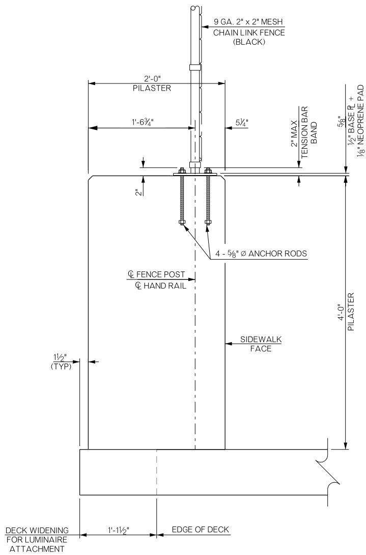
END VIEW OF WIDENED PILASTER AT PIERS 15 & 16
